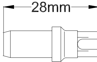
Modified Shuttle Spool (LHC P/N 8883031020)
